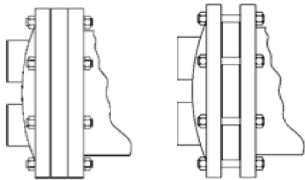
Full Face Boltless Tube Sheet
